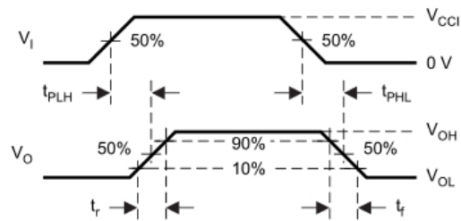
Figure 2.9 Switching Characteristics Test Circuit and Waveform
