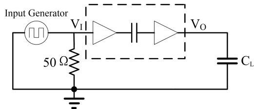
Figure 2.9 Switching Characteristics Test Circuit and Waveform
