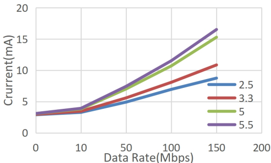
Figure 2.1 NSi8140 VDD1 Supply Current vs Data Rate
