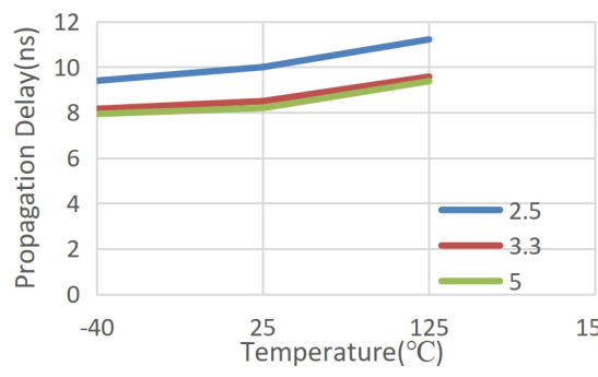
Figure 2.8 Falling Edge Propagation Delay Vs Temp
