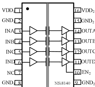
Figure 6.5 NSi8140W Package
