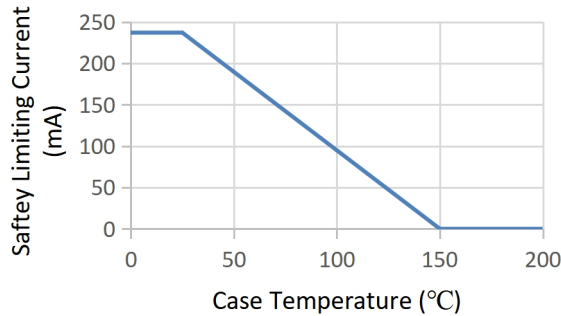
Figure 3.1 NSi8140N/NSi8141N/NSi8142N Thermal Derating Curve, Dependence of Safety Limiting Values with Case Temperature per DIN VDE V 0884-
