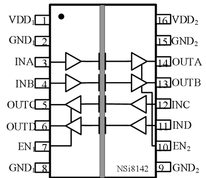
Figure 6.7 NSi8142W Package
